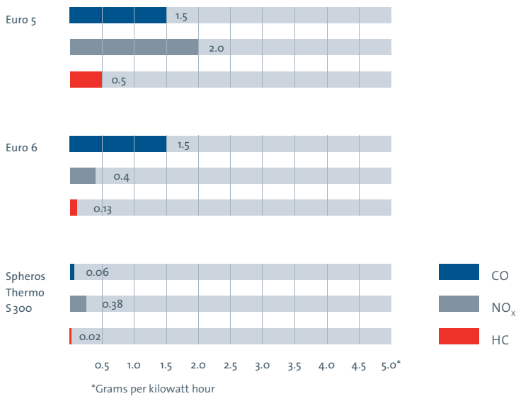
Exhaust emission values of Spheros Thermo S heaters compared to requirements for commercial vehicle combustion engines
